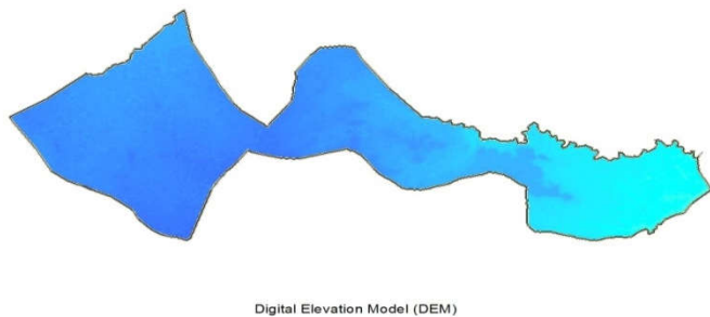
Figure 2 Digital Elevation Model of Basad Watershed Area
