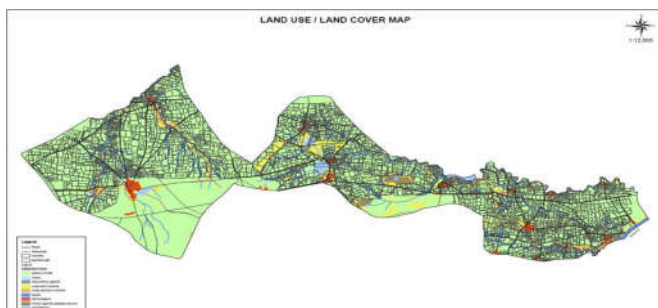
Figure 3 Land Use and Land Cover map of Basad Watershed Area
