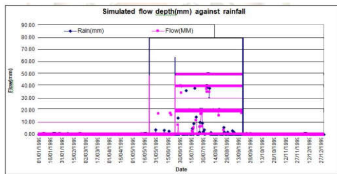
Figure 5 Simulated Flow depth against rainfall of Basad Watershed Area
