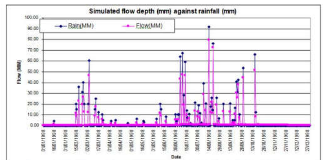
Figure 4 Simulated Flow depth against rainfall of Basad Watershed Area
