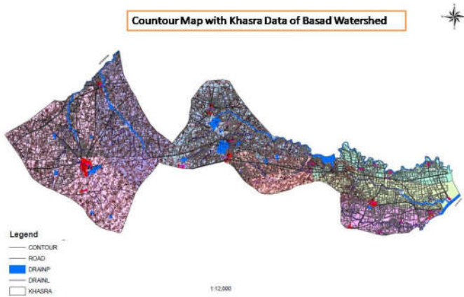
Figure 1 Contour Map of Basad Watershed Area
