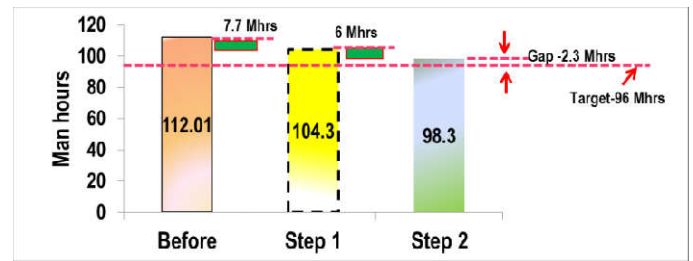
Chart 4 Effect of Muda elimination on man hours for overall main assembly process
