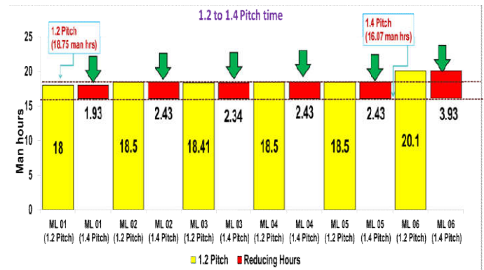
Chart 1 Current Man Hours Station wise and Man Hours
