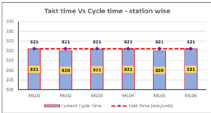
Chart 7 Takt time vs cycle time calculation after line-balancing
