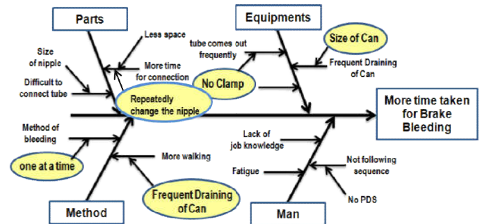
Chart 5 Analysis of cause of more time for Brake Bleeding Process
