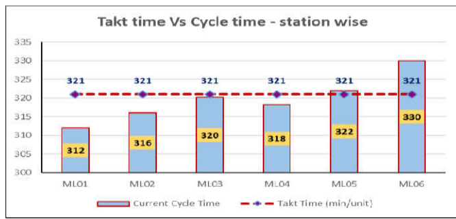
Chart 6 Takt-Time vs cycle time calculation and line balancing in each station of main assembly
