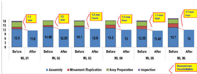
Chart 2 Effect of Kaizen on reduction of Man Hours in Assembly process – Station wise
