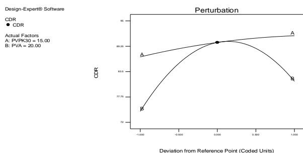
Fig No 10 Perturbation plot
