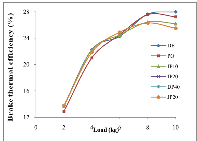
Fig 2 Variation of BTE with load
