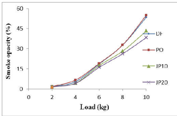
Fig 7 Variation of Smoke opacity with load
