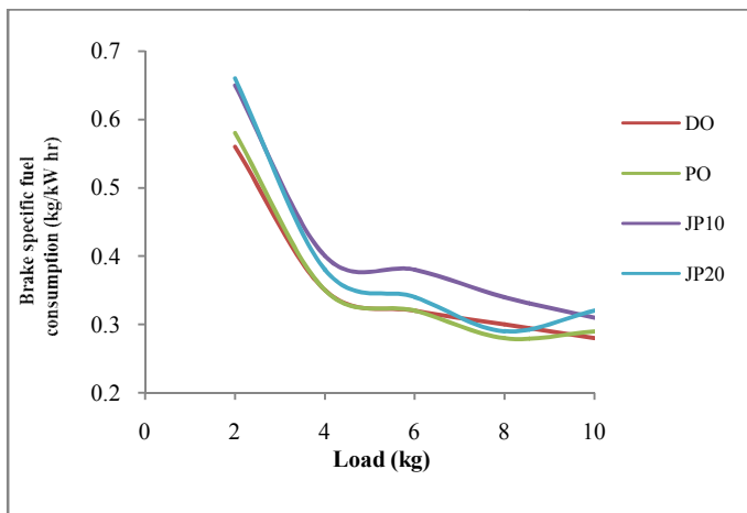
Fig 3 Variation of Bsfc with load
