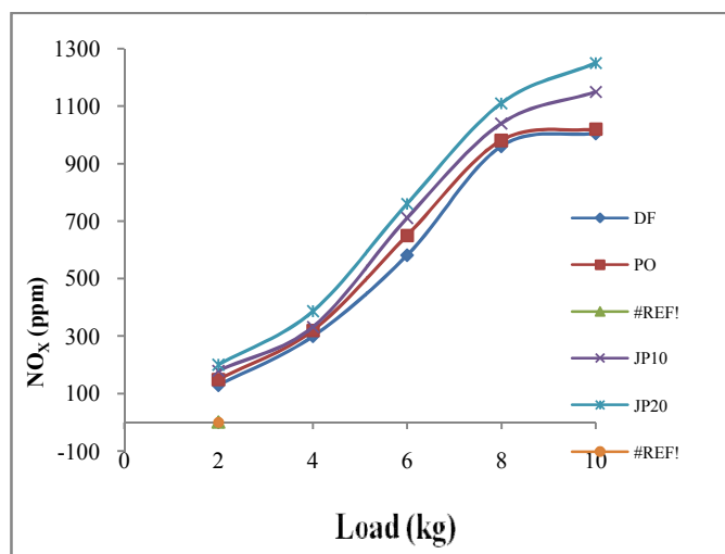
Fig 6 Variation of NOx with load
