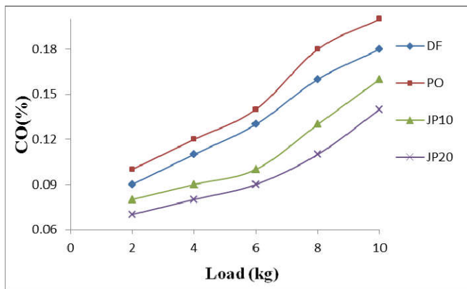
Fig 4 Variation of CO with load
